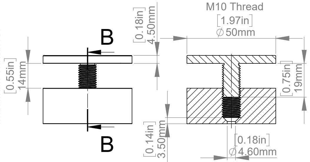
SECTION B-B SCALE 1 : 1.25
